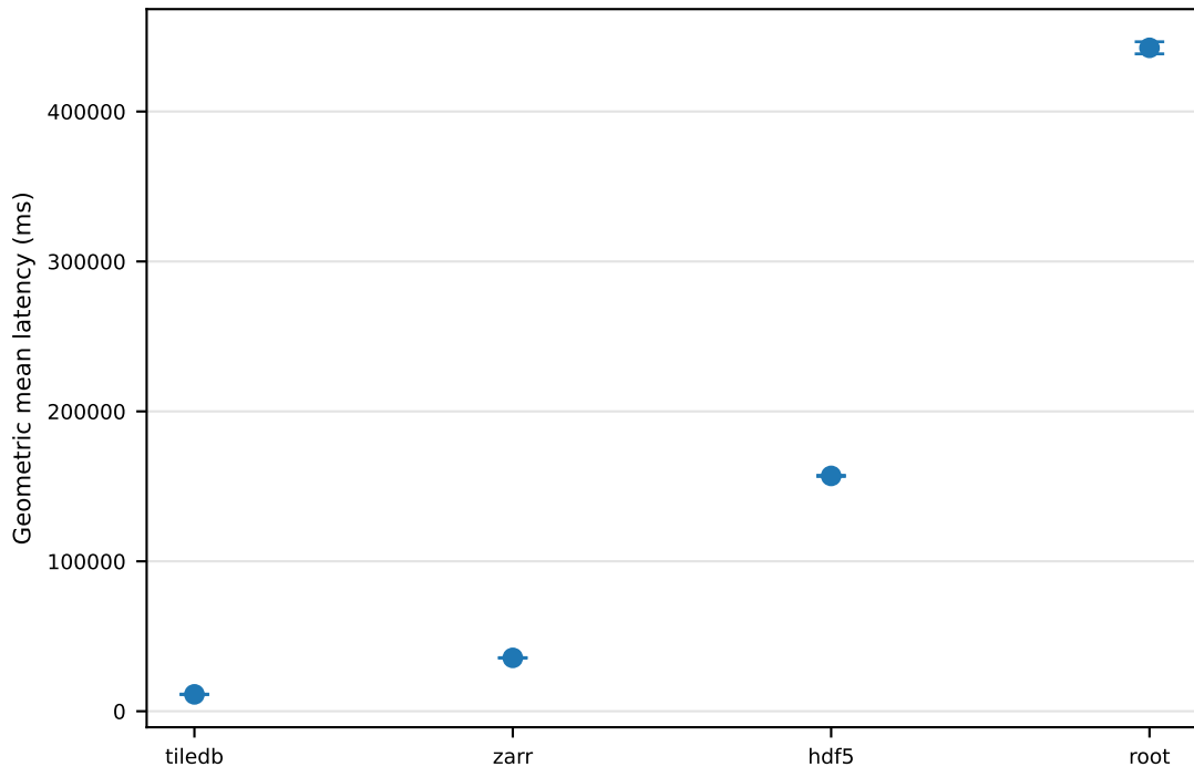
full latency — geometric mean \pm 95% CI, gzip
