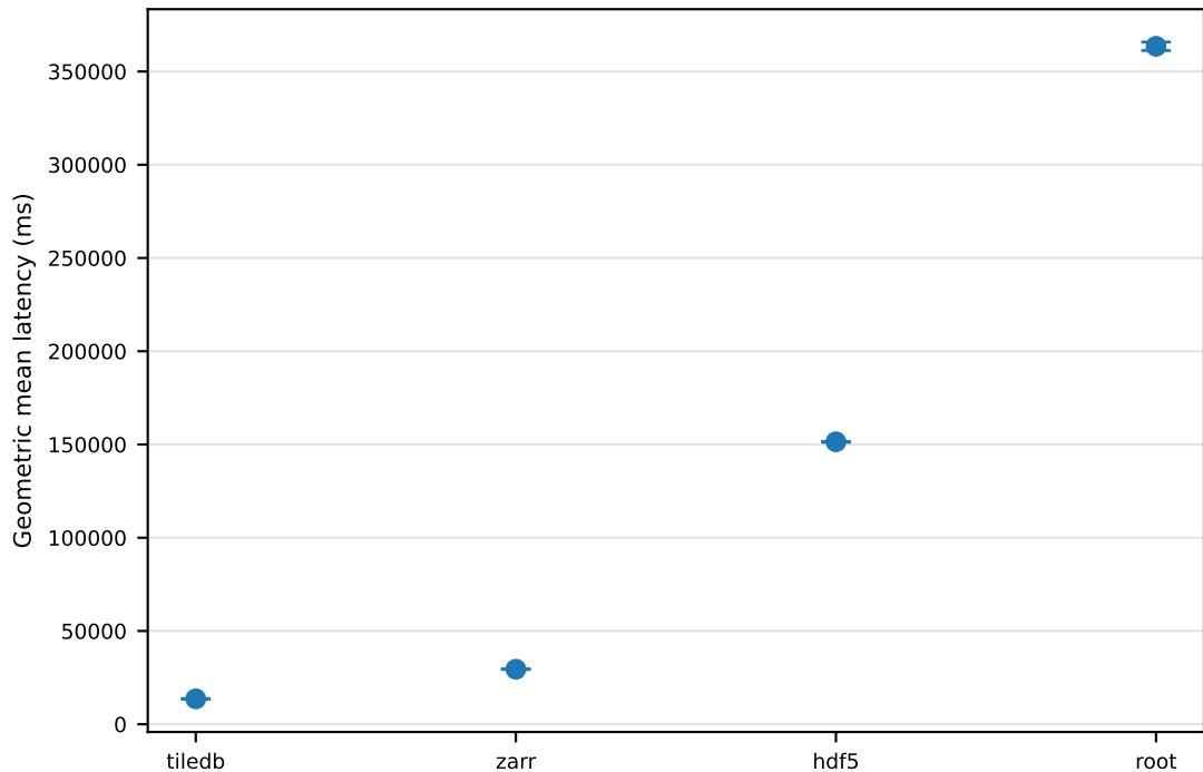
full latency — geometric mean \pm 95% CI, lz4
