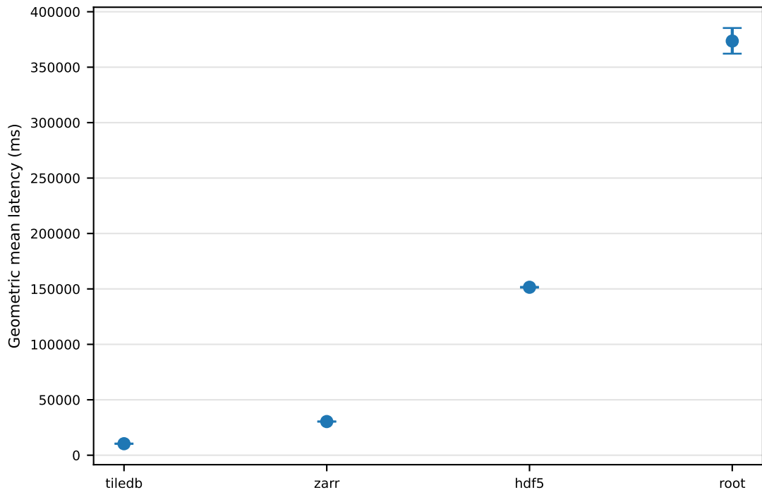
full latency — geometric mean \pm 95% CI, zstd
