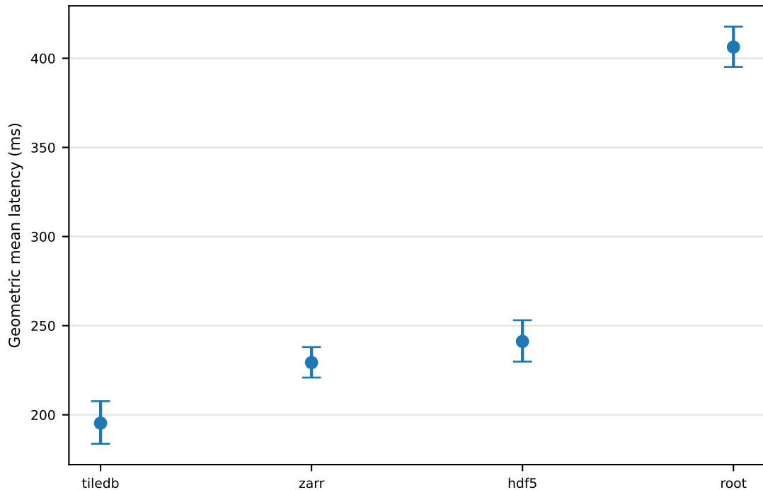
slice latency — geometric mean \pm 95% CI, gzip
