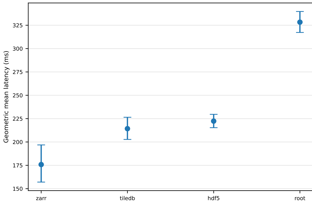
slice latency — geometric mean \pm 95% CI, lz4
