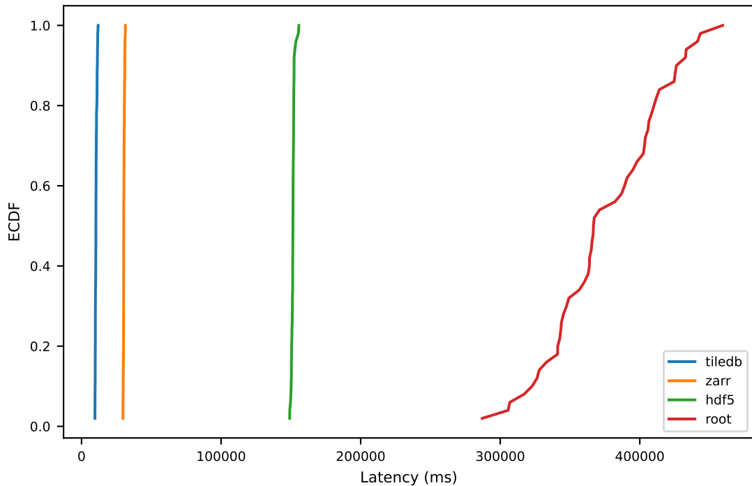
full latency — ECDF, zstd
