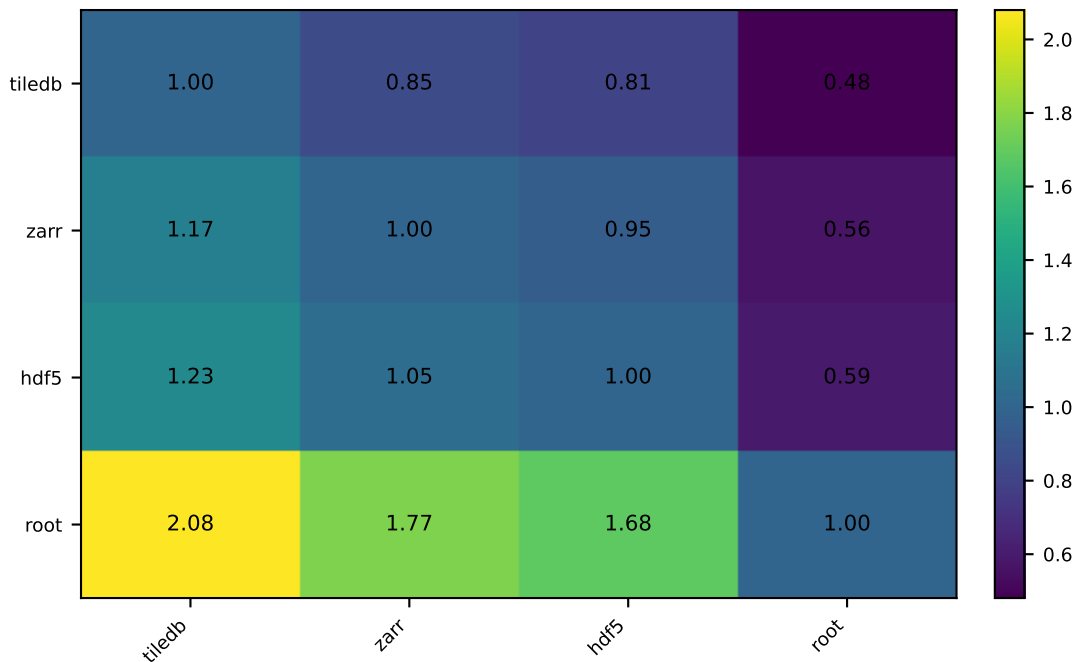
Pairwise time ratios (row / column) — gzip slice <1 means row faster
