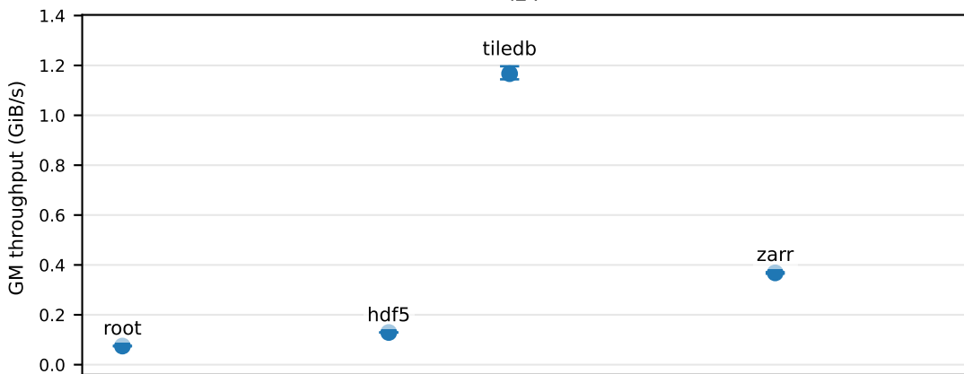
zstd
