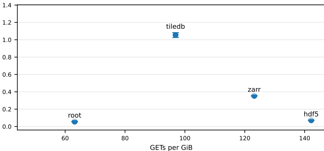
zstd
