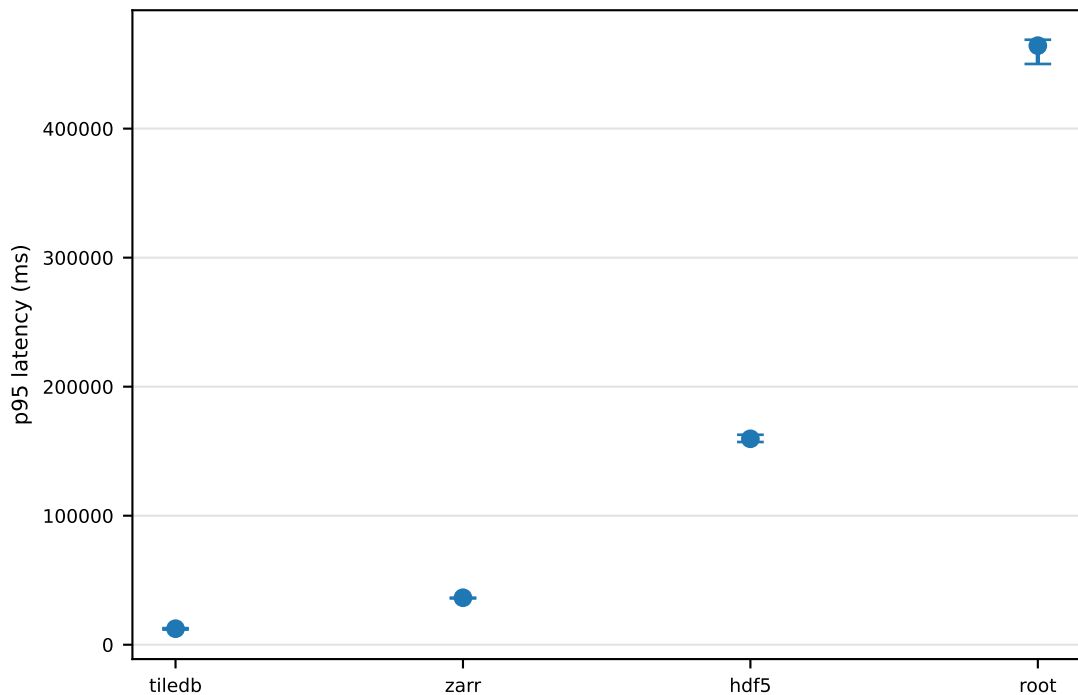
full — gzip: p95 latency \pm 95% CI (block bootstrap)
