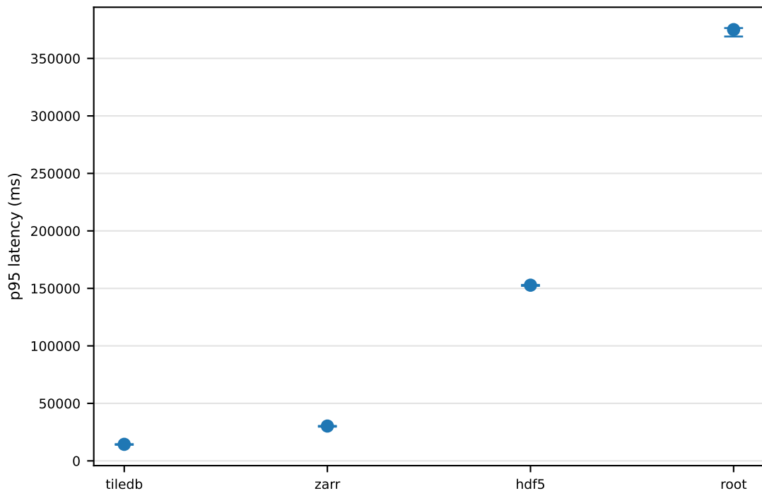
full — lz4: p95 latency \pm 95\% CI (block bootstrap)
