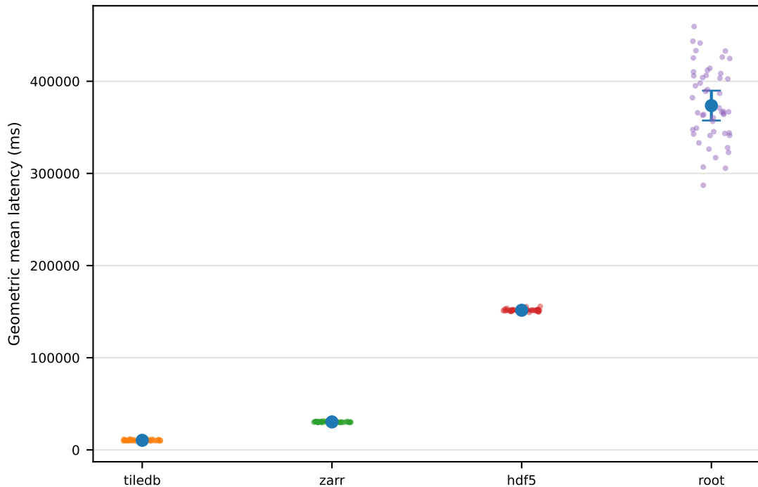
full — zstd: GM latency \pm 95\% CI (dependence-robust)
