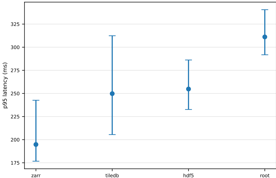
slice — zstd: p95 latency \pm 95% CI (block bootstrap)
