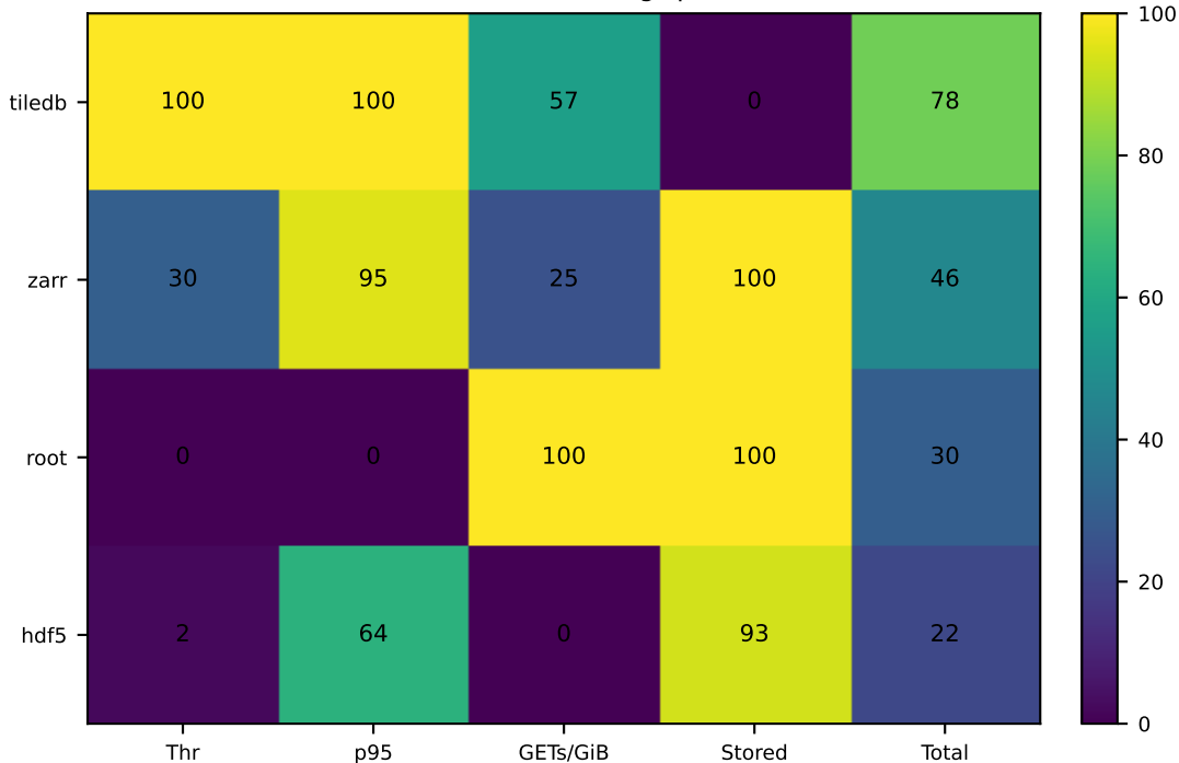
Scores (Full) — gzip
