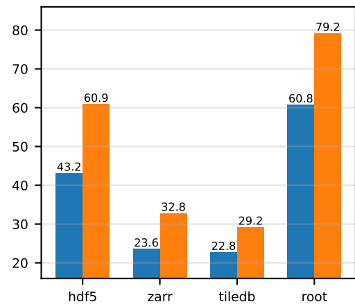
zstd / full
