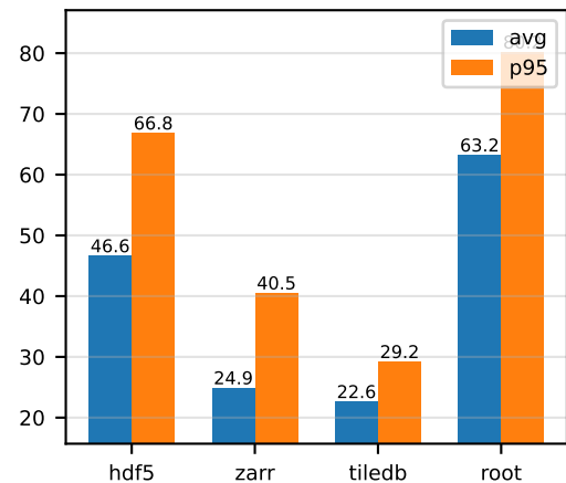
lz4 / full
