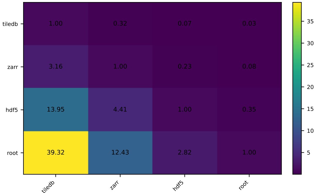
Pairwise time ratios (row / column) — gzip full <1 means row faster
