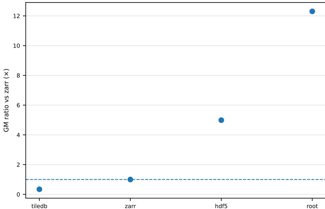
full — zstd: Descriptive GM ratios (session-conditional)
