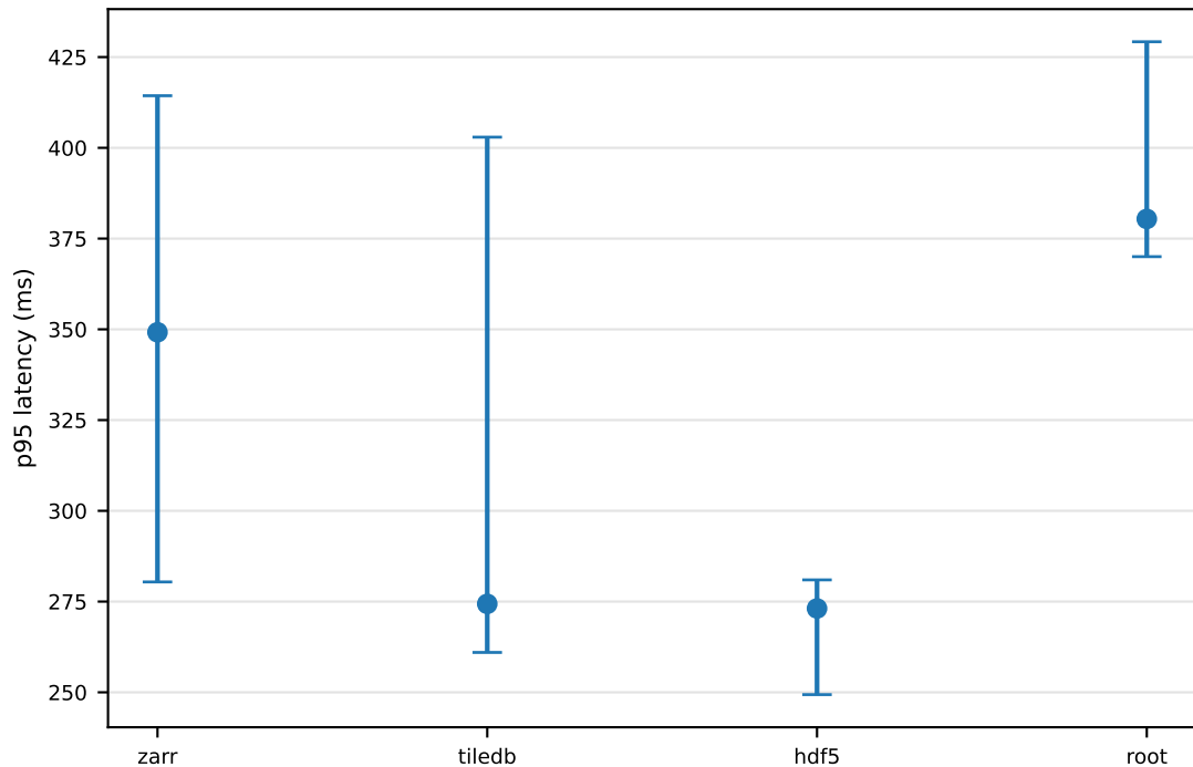
slice — lz4: p95 latency \pm 95\% CI (block bootstrap)
