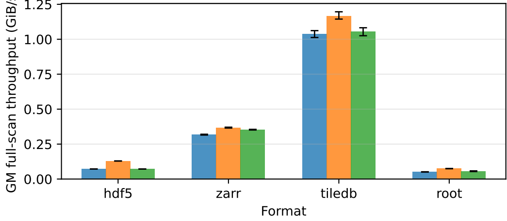
Full-scan throughput (higher is better)
