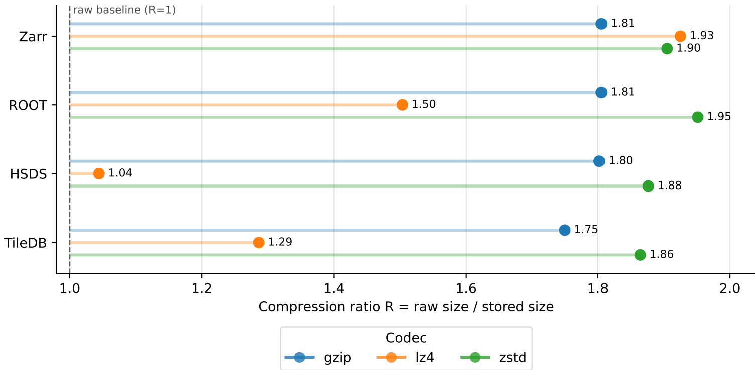
Compression ratio by format and codec (higher is better)
