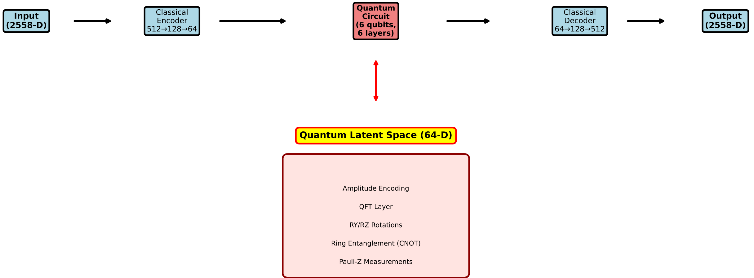
Hybrid Quantum-Classical Variational Autoencoder
