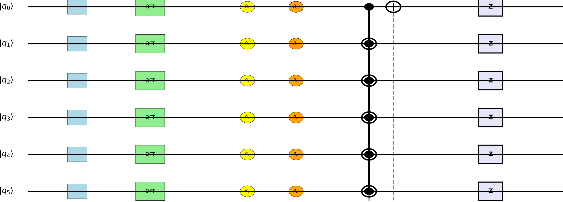
6-Qubit Parameterized Quantum Circuit
