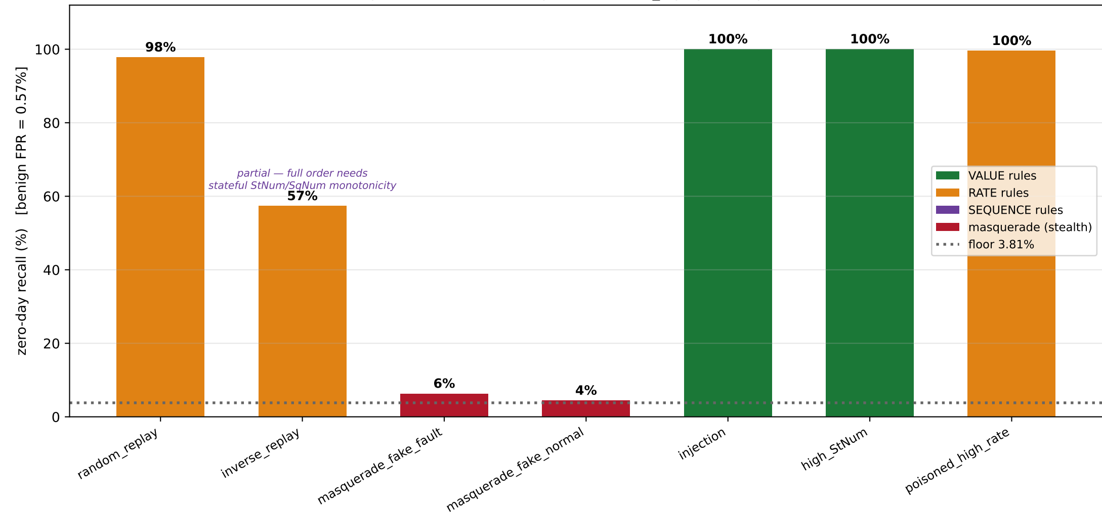
Zero-day by protocol spec: VALUE + RATE + SEQUENCE rules (benign-only, zero examples): rate solved (poisoned 100%); order partial (inverse_replay); masquerade irreducible
