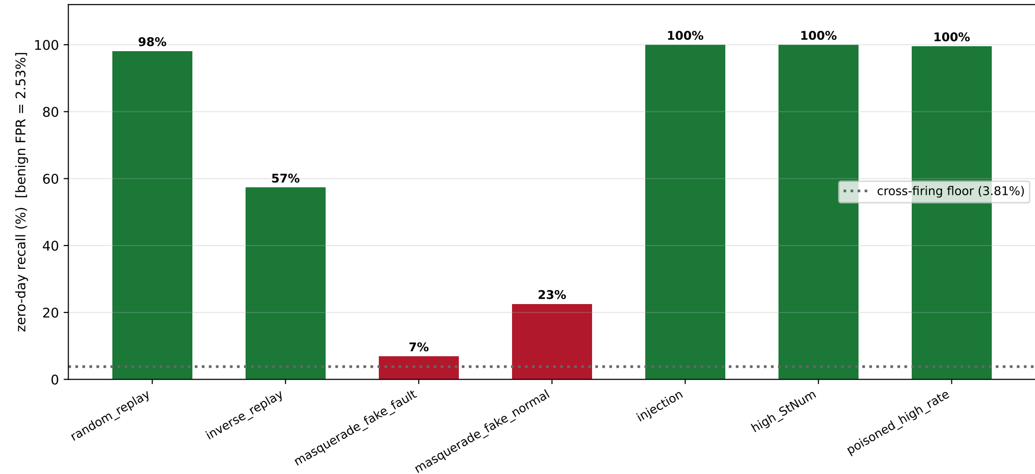
Benign-spec rules over ALL features (zero attack examples): does ERENO encode the rate/sequence signal per-sample?
