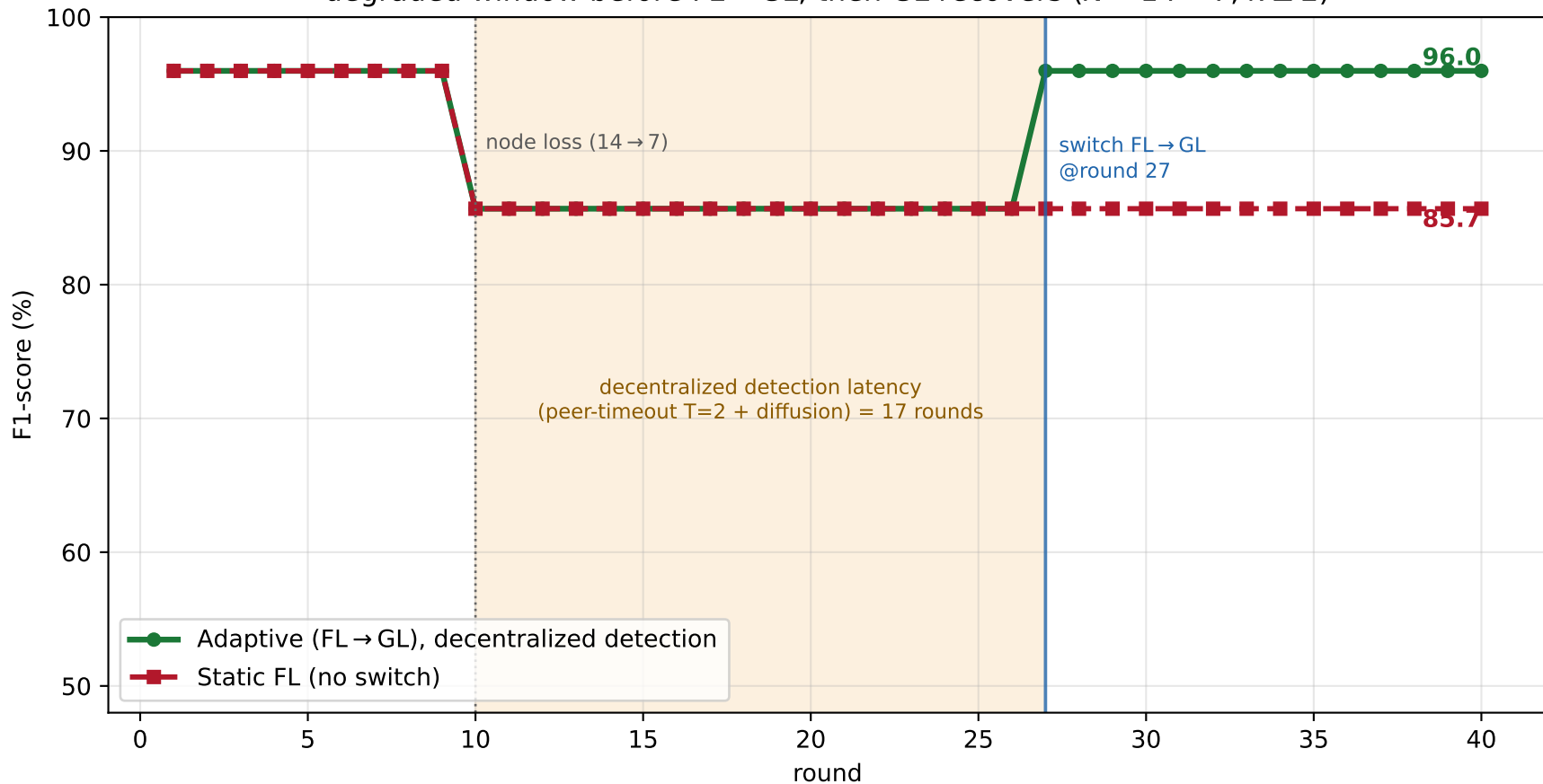
Latency-aware end-to-end (composition): decentralized detection adds a degraded window before FL \rightarrow GL, then GL recovers ( N = 14 \rightarrow 7 , k \geq 2 )
