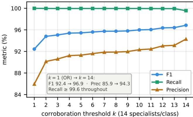
(a) Precision-recall vs. k ( N = 98 )
