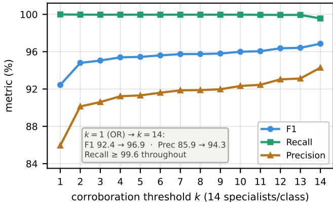
Precision-recall vs. k ( N = 98 )
