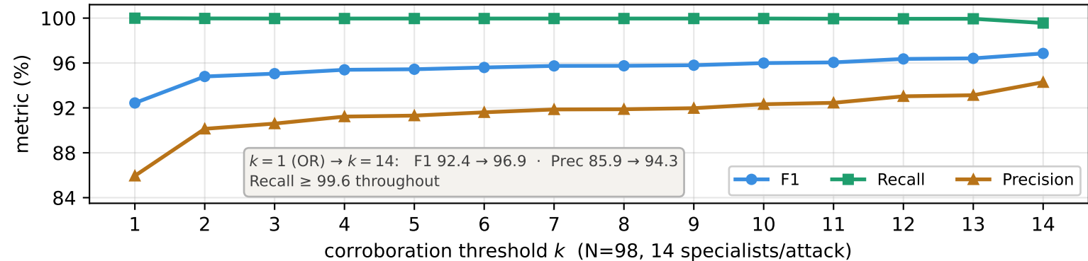
N=98 (14 specialists/attack): precision-recall frontier over k
