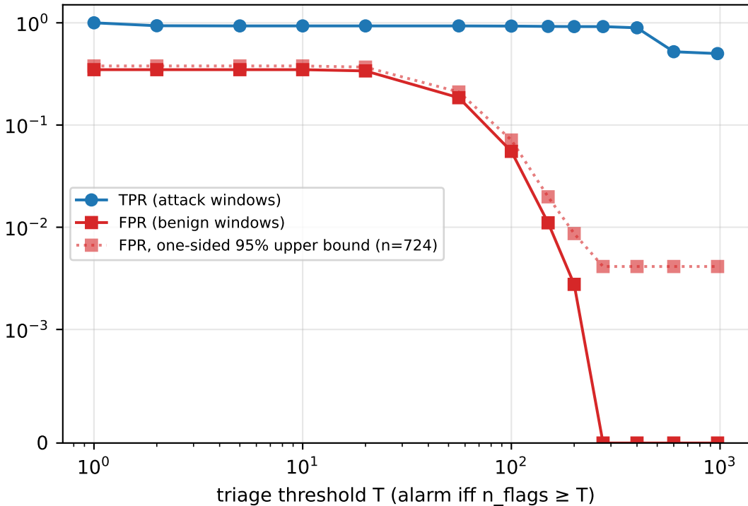
Window-level rates vs triage threshold
