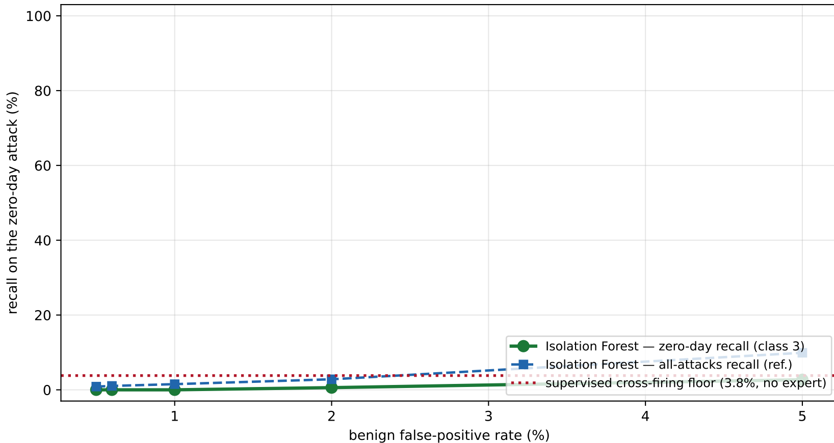
Off-the-shelf anomaly detection (Isolation Forest) on the GRASP features FAILS to detect this zero-day: recall stays at/below the cross-firing floor
