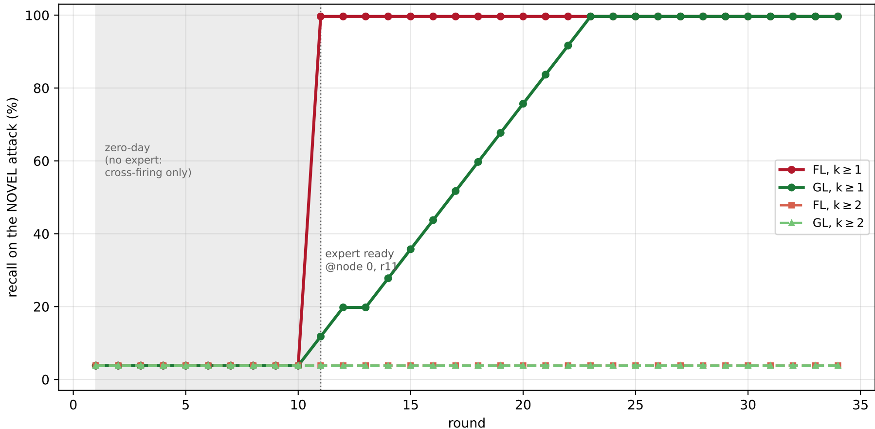
Convergence to a NOVEL attack, SINGLE source ( N = 12 , 2/attack, ring): FL k \geq 1 \sim 1 round; GL k \geq 1 diffuses; k \geq 2 stays low (RQ4: needs a 2nd expert)
