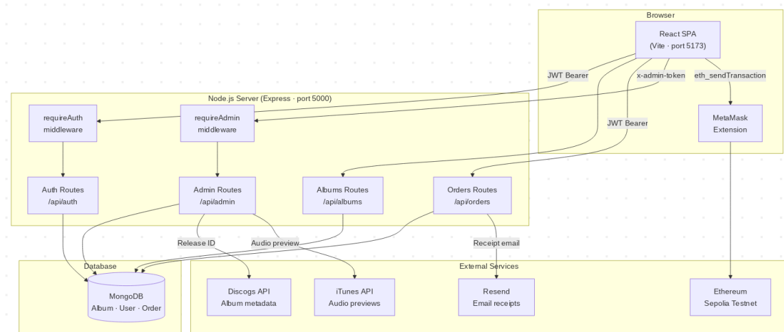
Figure 4.1: System architecture overview
