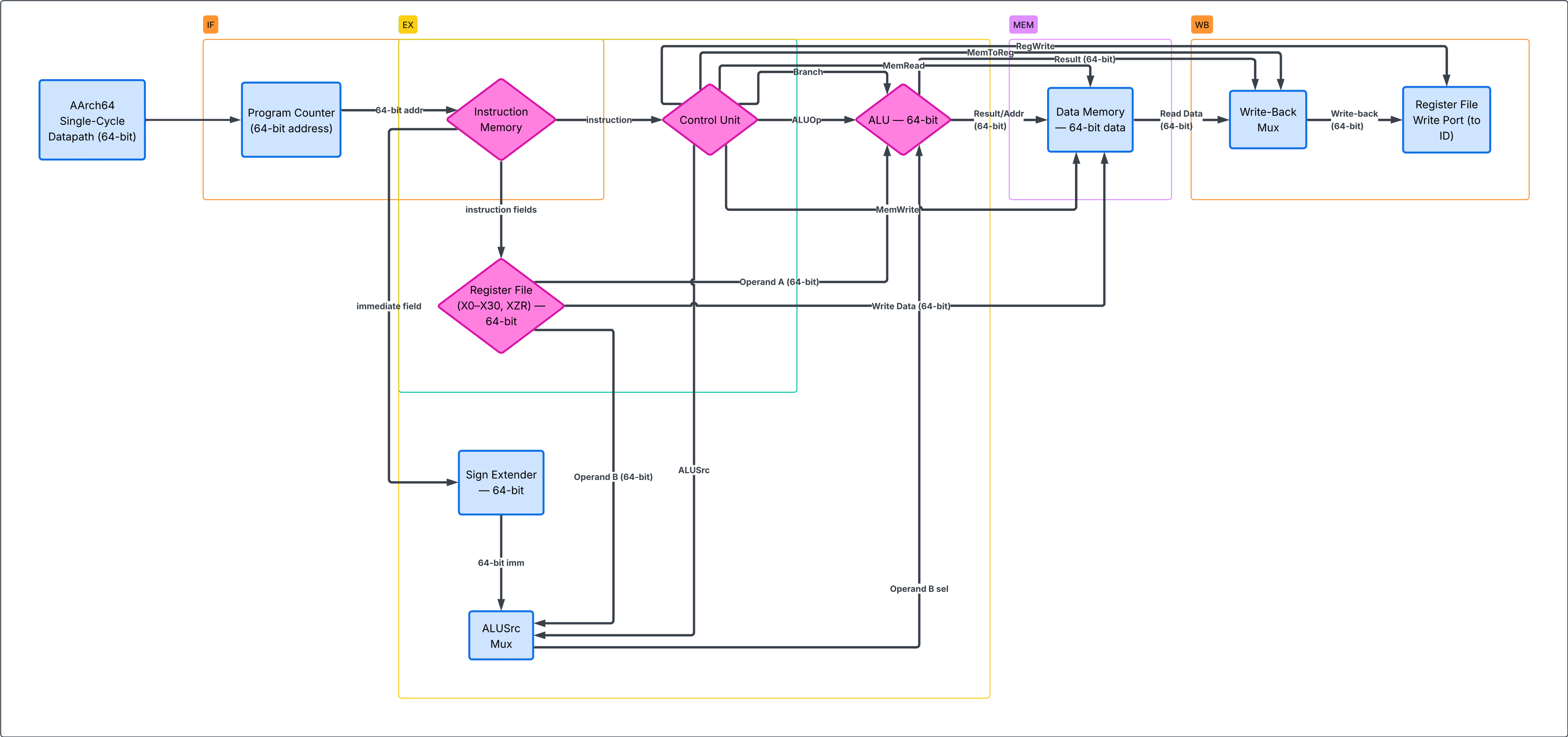
AArch64 Single-Cycle Datapath Diagram
