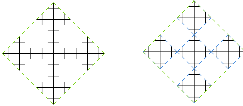
Diagram 1.1: The opens sets V (green) and \mathcal{S}_i(V) (blue)
