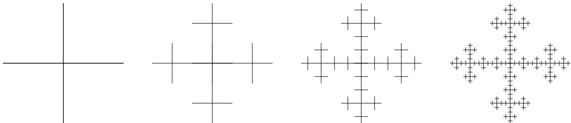
Diagram 1.1: Vicsek graph, G_0, G_1, G_2 and G_3
