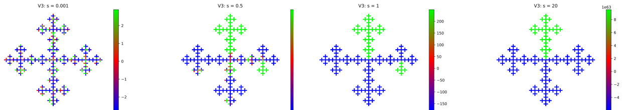
Figure 5.3: Simulations of the Vicsek set on V_3 with different s parameters and with the same white noise. A larger version of the image can be found in Appendix A
