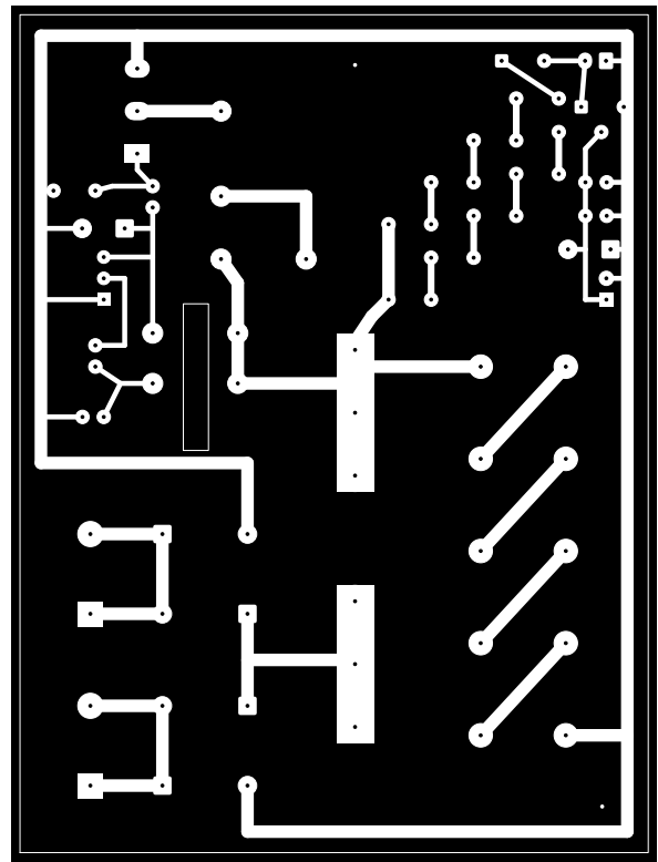
B.Cu NEGATIVE (white = copper)
