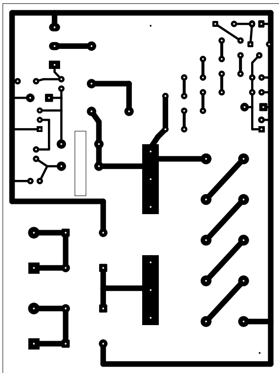
B.Cu POSITIVE (black = copper)
