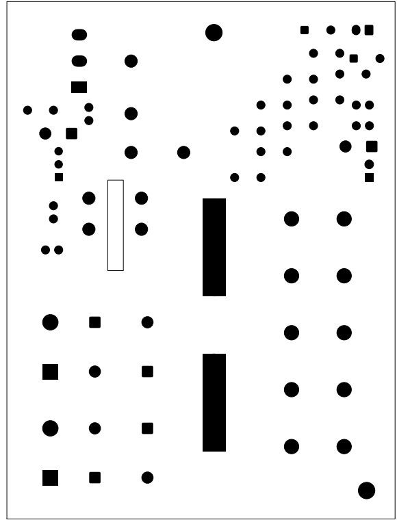
B.Mask (black = pad openings)
