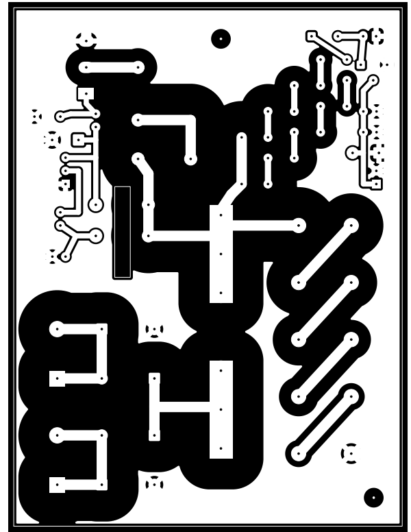
B.Cu NEGATIVE (white = copper)
