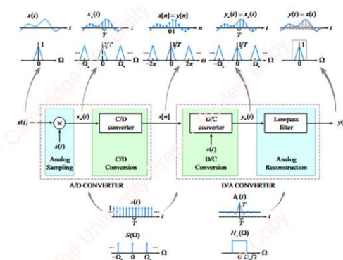
Figure 6.28 Summary of A/D and D/A conversion
