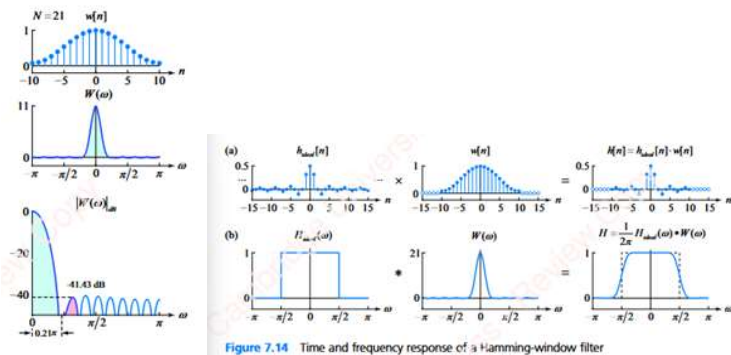
Figure 7.14 Time and frequency response of a Hamming-window filter
