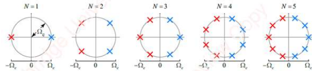
Figure 8.5 Poles of the Butterworth filter
