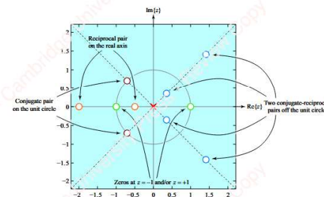
Figure 4.15 Position of zeros for linear-phase FIR systems
