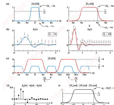
Figure 8.16 Impulse-invariance example
