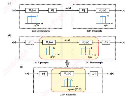
Figure 6.47 Resampling
