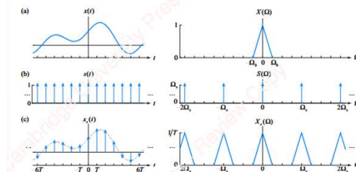
Figure 6.5 Analog sampling
