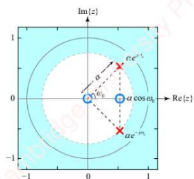
Figure 4.13 Pole-zero plot of a second-order system
