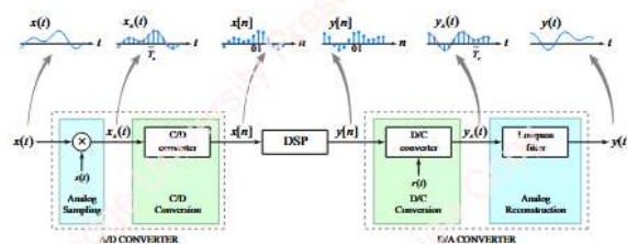
Figure 6.2 Model of the digital signal processing paradigm
