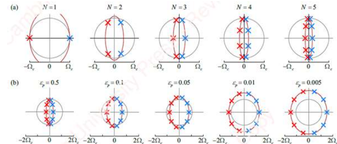
Figure 8.9 Poles of a Chebyshev filter
