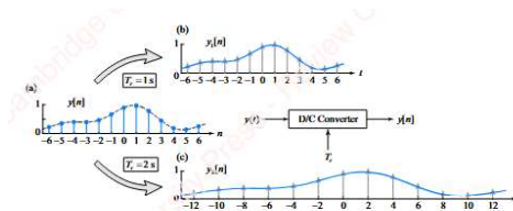
Figure 6.27 Discrete-to-continuous (D/C) converter
