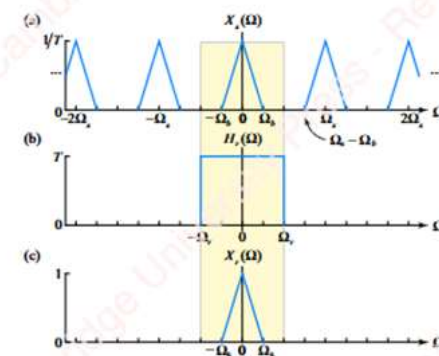
Figure 6.6 Recovery of X_r(Ω) from X_s(Ω) by lowpass filtering
