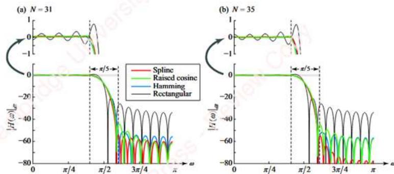
Figure 7.30 Spline and raised-cosine filters
