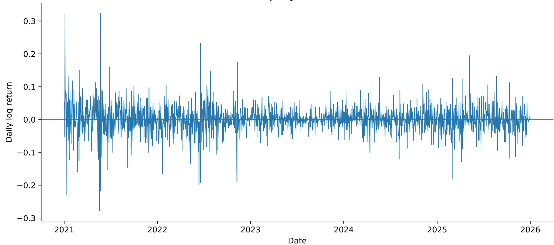
Ethereum Daily Log Returns, 2021-2025
