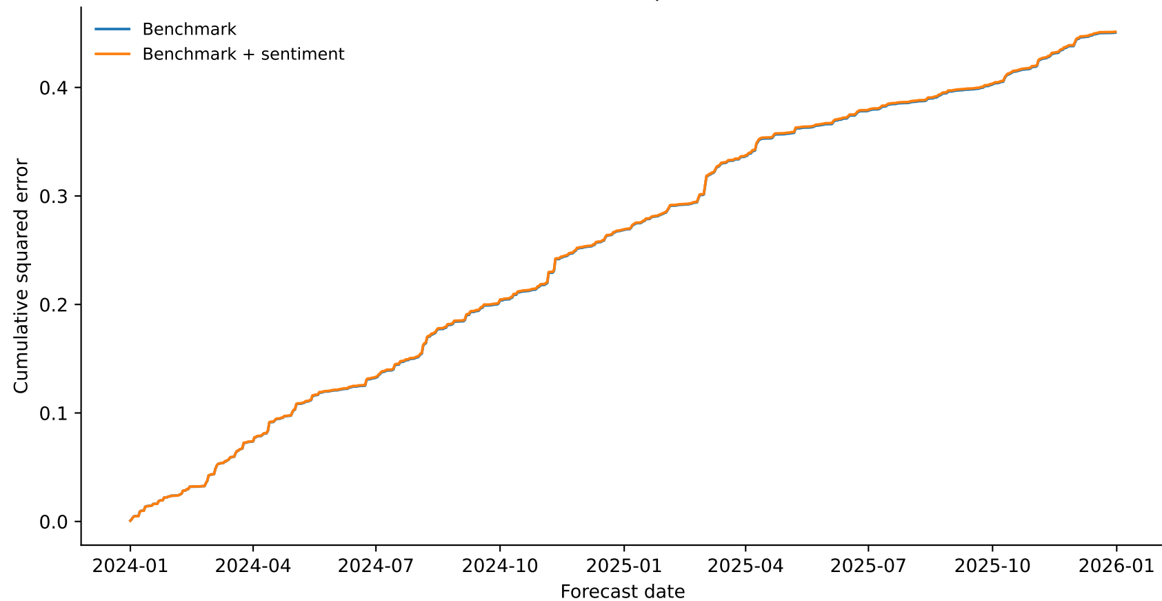
Bitcoin Cumulative OOS Squared Forecast Error
