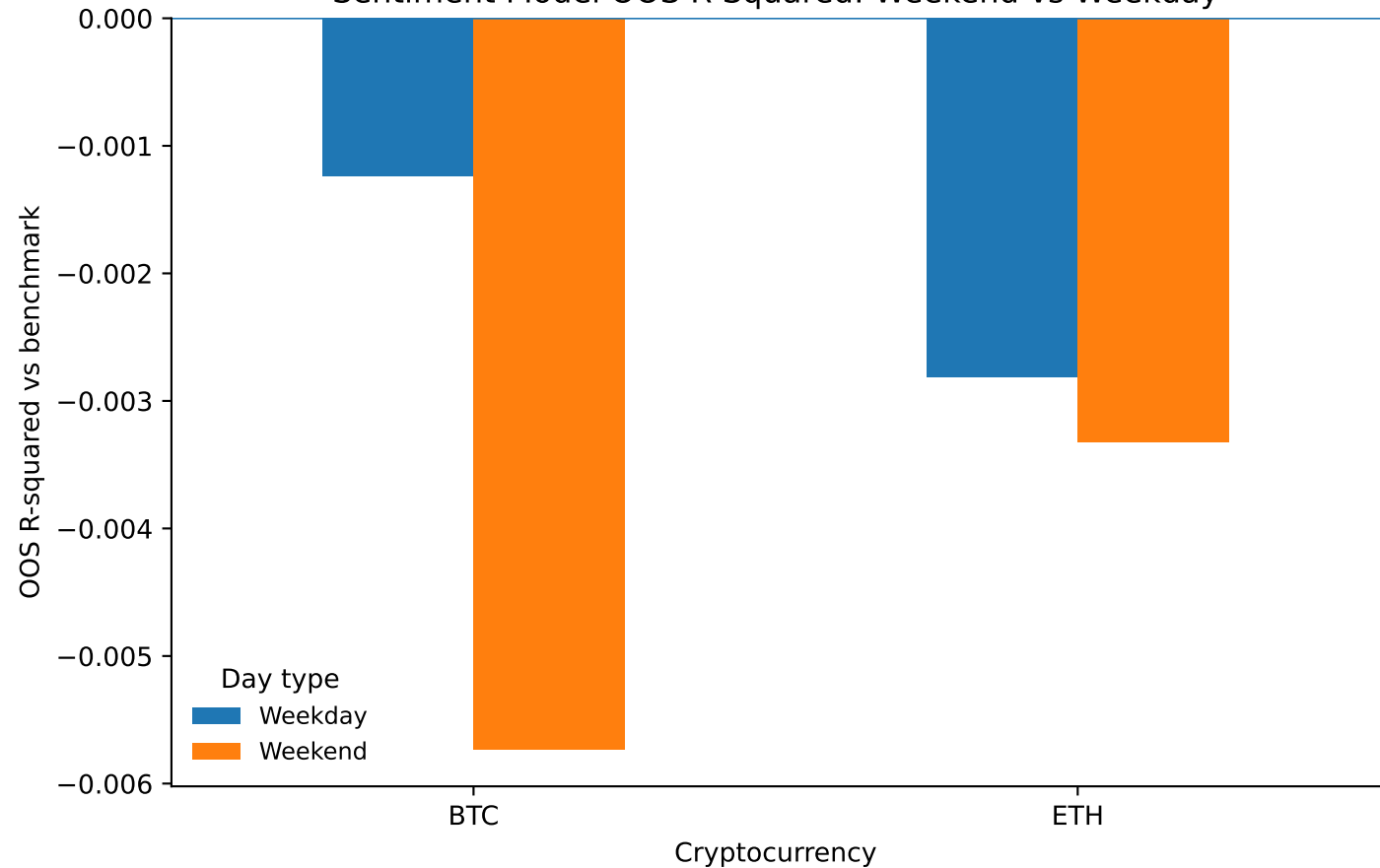
Sentiment Model OOS R-Squared: Weekend vs Weekday
