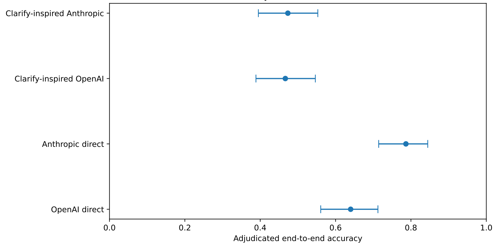
Final accuracy with 95% Wilson intervals
