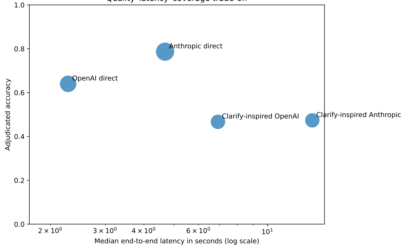
Quality-latency-coverage trade-off
