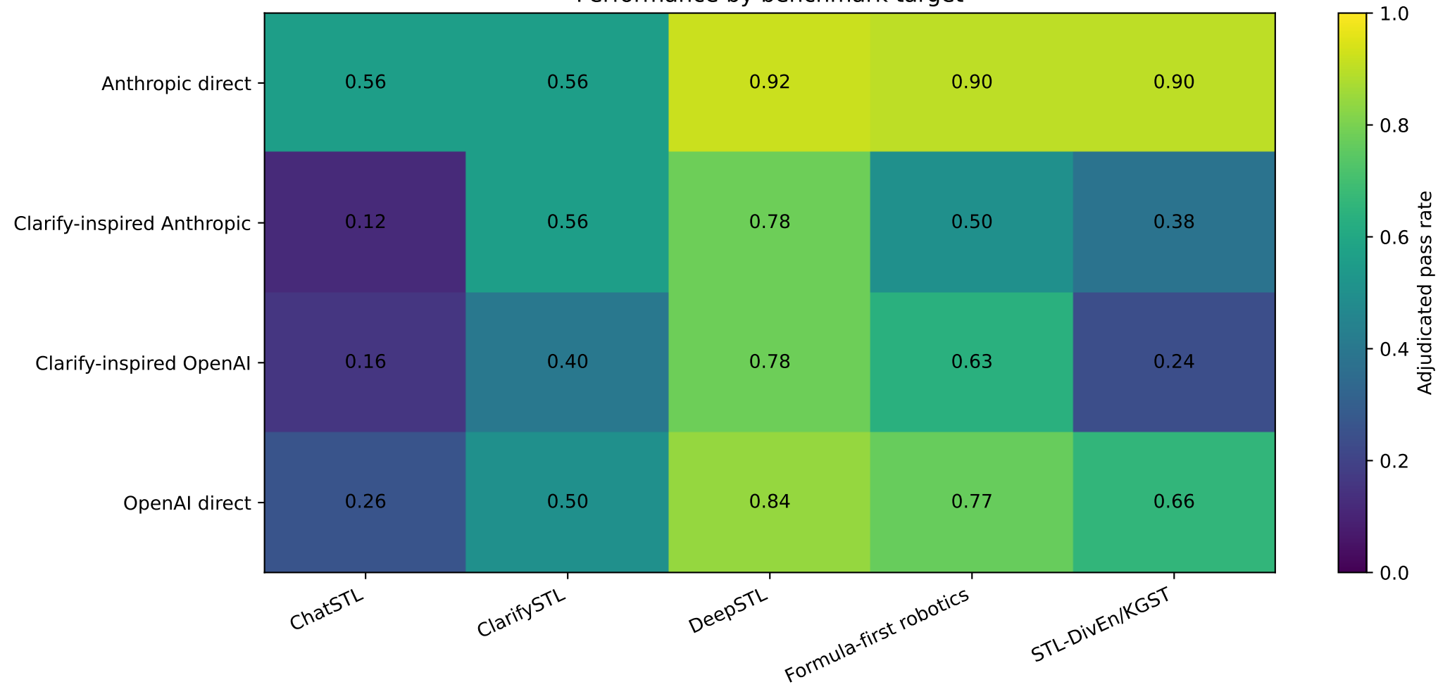
Performance by benchmark target
