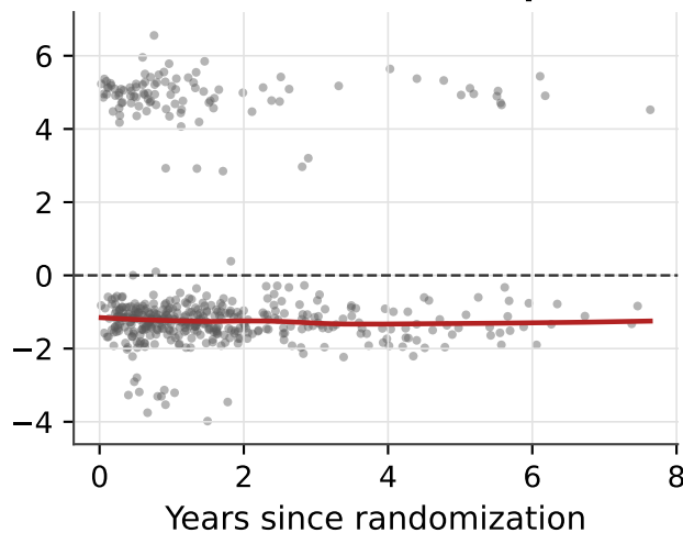
Obstruction (PH violation, p = 0.008 )
