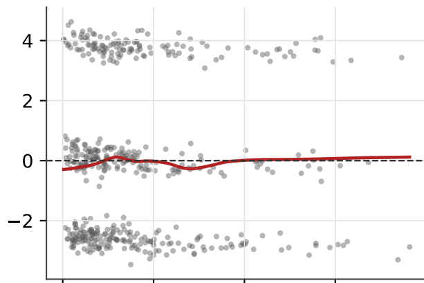
Obstruction (PH violation, p = 0.008 )
