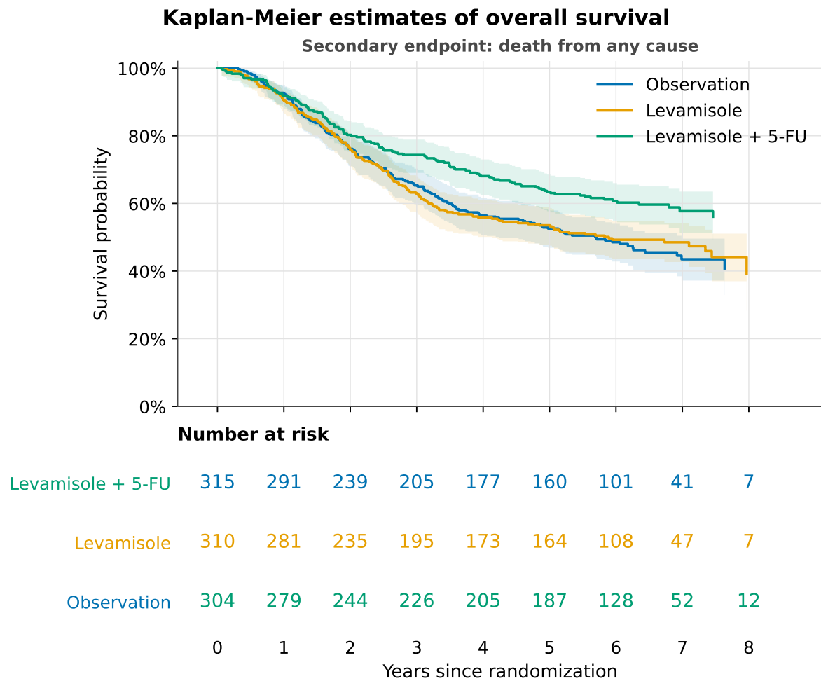
Figure 2: Kaplan–Meier estimates of overall survival (secondary endpoint) with pointwise 95% confidence bands and numbers at risk.
