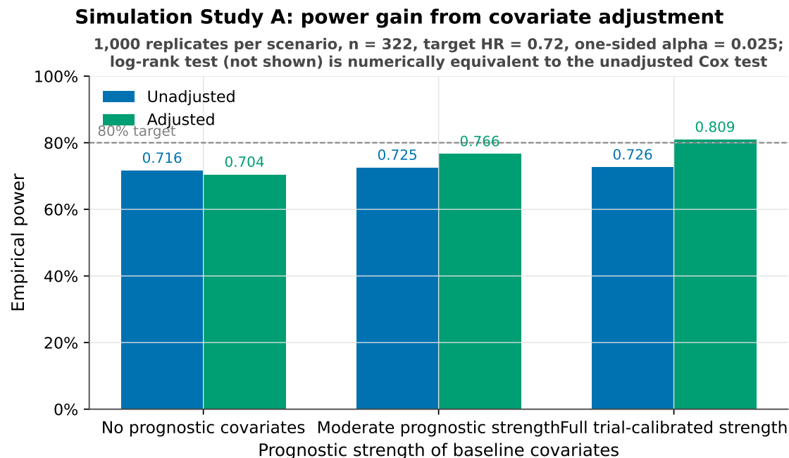
Figure 10: Simulation Study A: empirical power of the unadjusted versus covariate-adjusted Cox test as a function of prognostic strength (target HR 0.72, n = 322 , 1,000 replicates per scenario).
