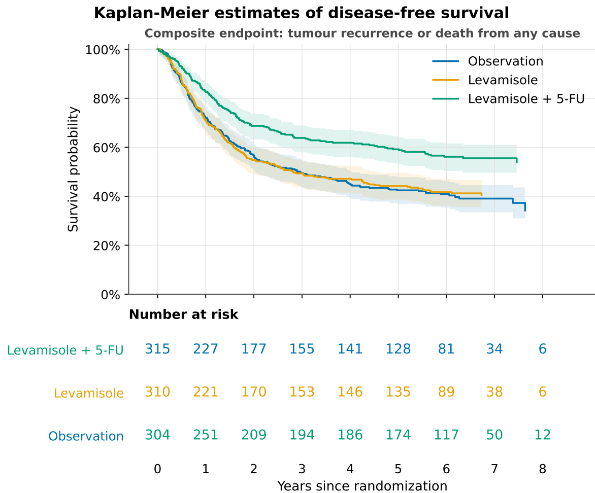
Figure 1: Kaplan–Meier estimates of the composite disease-free survival endpoint (primary) with pointwise 95% confidence bands and numbers at risk.
