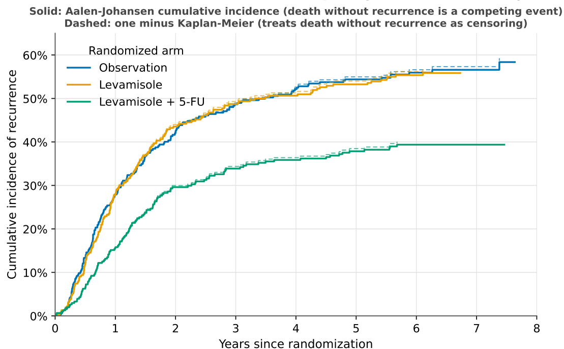
Figure 5: Cumulative incidence of recurrence: Aalen-Johansen estimates treating death without recurrence as a competing event (solid) versus the naive one-minus-Kaplan-Meier estimator that censors such deaths (dashed).
