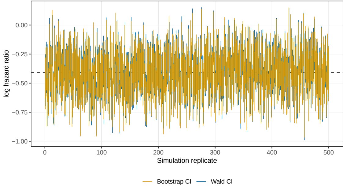
Figure 12: Simulation Study C: Wald versus bootstrap percentile intervals for the log hazard ratio across 500 simulated trials under a time-varying true effect. The dashed line marks the simulation estimand.
