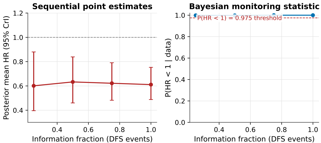
Figure 16: Bayesian sequential monitoring under the skeptical prior. Left: posterior mean hazard ratio with 95% credible intervals at each look. Right: the monitoring statistic P(HR < 1) against the 0.975 stopping threshold.
