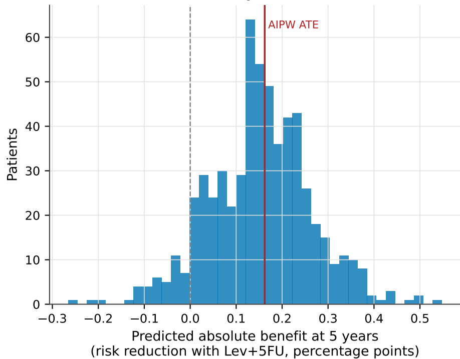
Distribution of predicted benefit
