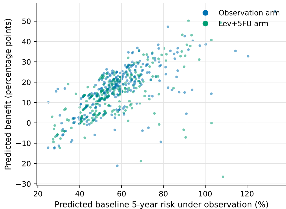
Benefit versus baseline risk
