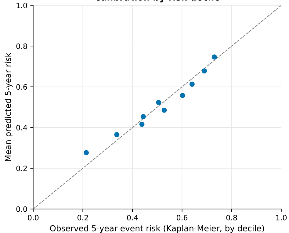
Calibration by risk decile
