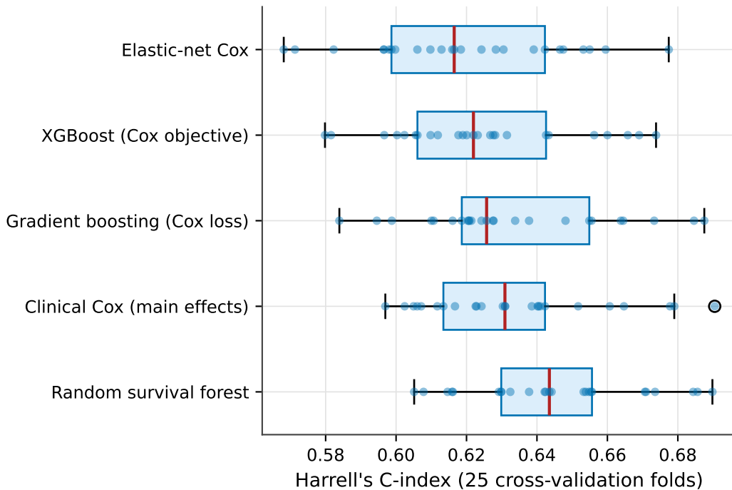
Discrimination: cross-validated
