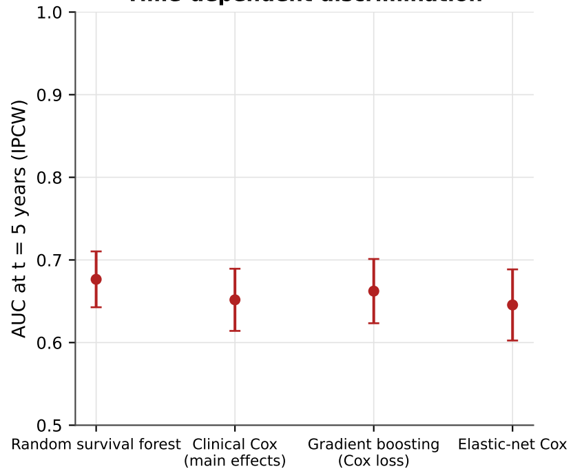
Time-dependent discrimination
