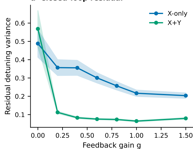
d Closed-loop residual
